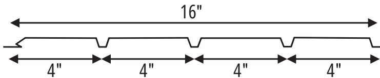
3/8" F-Trim (Aluminum)
