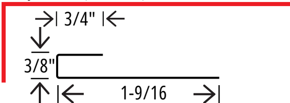
1/2 J-Channel (Aluminum)
