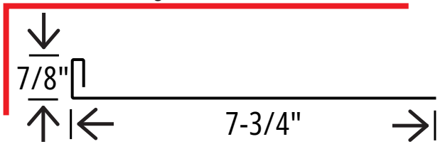
Aluminum Trim Coil 18 3/4"
